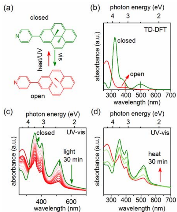
Figure 1. Ring opening/closure of the Py-DHP switch. Switching between the two isomers in Figure 1a can be triggered by visible light (ring opening) and heat or UV-light (ring closure). The ring opening process of the Py-DHP film (10 nm) reaches a photothermal equilibrium after ca. 30 min illumination ( \lambda = 565 nm, I_{\max} > 200 mW cm -2 ) and can be reset by heat treatment (50 °C), as displayed by UV-vis absorption spectra in Figures 1c and 1d. Calculated absorption spectra of Py-DHP by time-dependent DFT (TD-DFT) are also plotted in Figure 1b for sake of a comparison.
