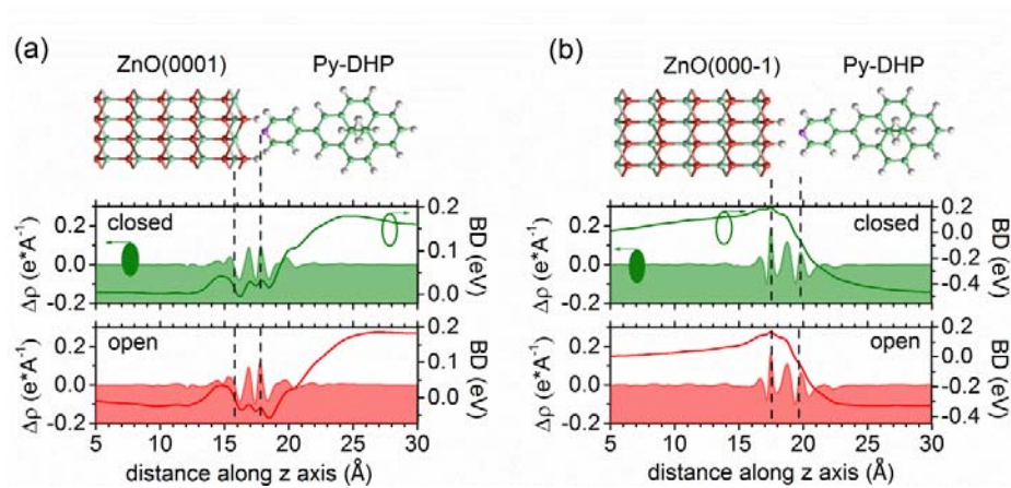
Figure 4. Plane averaged charge density difference ( \Delta\rho ) and corresponding bond dipole (BD) potential for (a) Py-DHP on ZnO(0001) and Py-DHP on ZnO(000-1), respectively. The positions of the topmost Zn or O layer in ZnO and the N layer in Py-DHP are indicated by the vertical dashed lines.
