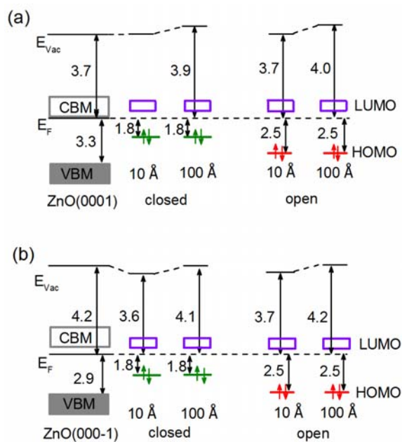
Figure 3. Schematic energy level diagram of (a) Py-DHP/ZnO(0001) and (b) Py-DHP/ZnO(000-1) interfaces. All values are in the unit of eV. Energy positions of vacuum level ( E_{vac} ), VBM, HOMO with respect to the Fermi level ( E_F ) are derived from UPS measurements.
