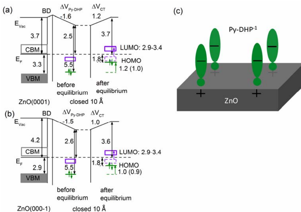
Figure 5. Fermi level pinning of closed Py-DHP on (a) ZnO(0001) and (b) ZnO(000-1). Before equilibrium, the frontier levels of Py-DHP are located below the Fermi level due to the potential drop created by the intramolecular dipoles. After equilibrium, HOMO levels of closed Py-DHP are located at 1.8 eV below the Fermi level. This corresponds to 1.2 eV and 1.0 eV upshifts of negatively charged Py-DHP (Py-DHP -1 ) levels on ZnO(0001) and ZnO(000-1), respectively. The mapping of electrostatic potential in the uncharged Py-DHP region shows ca. 1.0 eV (shown in the parentheses) potential increase, which agrees well with the measured HOMO onset. (c) Schematic illustration of the Py-DHP -1 molecules on ZnO, while the surrounding neutral Py-DHP is not shown.
