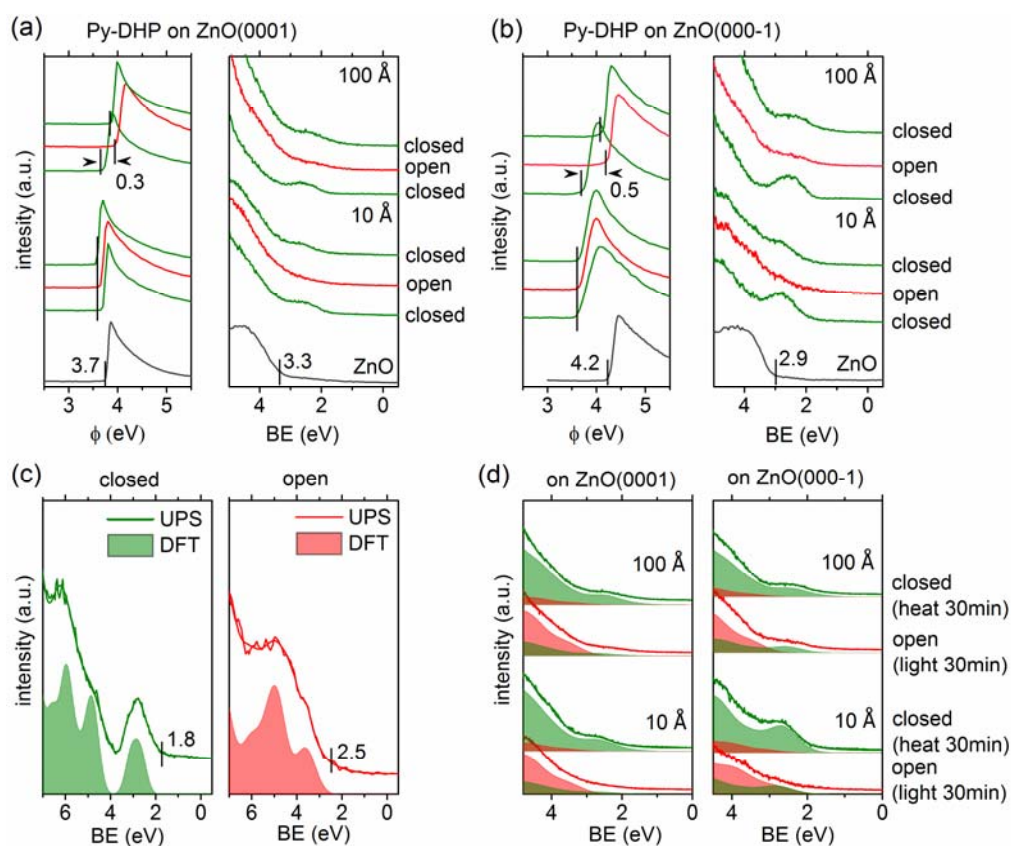
Figure 2. UPS spectra of 10 Å and 100 Å Py-DHP films evaporated on (a) ZnO(0001) and (b) ZnO(000-1) surfaces. For each film, in situ switching was realized through the illumination by green light (565 nm), which switches the molecule from the closed to the open form (red line); and through heating at 50 °C for switching back to its closed form (green line). (c) UPS spectra (substrate signal subtracted) and DFT calculated density of states (DOS) of the closed and open Py-DHP molecules. The DFT calculated spectra were shifted by 0.4 eV for aligning the experimental results. In the calculations, photoemission cross sections have not been taken into account. (d) Decomposition of the sample spectra into closed and open Py-DHP contributions.
