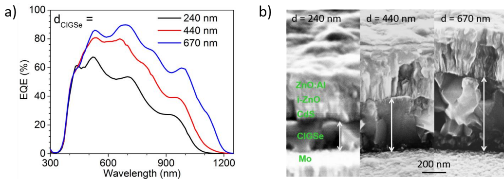
Figure 2. a) External quantum efficiency of thin-film \text{Cu}(\text{In,Ga})\text{Se}_2 solar cells with an absorber thickness of 240 nm, 440 nm and 670 nm, b) cross sectional SEM images of the solar cells with various absorbers thicknesses.
