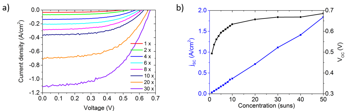
Figure 6. Electrical measurements of circular CIGSe micro solar cells sized 425 \mu\text{m} in diameter and obtained in a top-down approach: a) jV characteristics for various concentration factors, b) j_{\text{sc}} and V_{\text{oc}} as a function of concentration.
