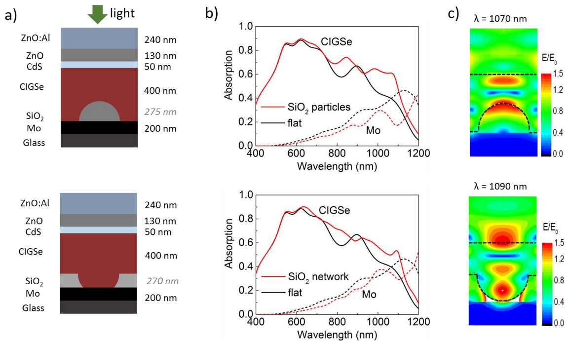
Figure 3. Simulation of CIGSe solar cells with integrated \text{SiO}_2 hemispherical nanoparticles (top row) and \text{SiO}_2 network (bottom row): a) schematic solar cell structure, b) calculated absorption of CIGSe and Mo back contact as compared to the flat reference, c) electric near-field distribution at the major resonance.
