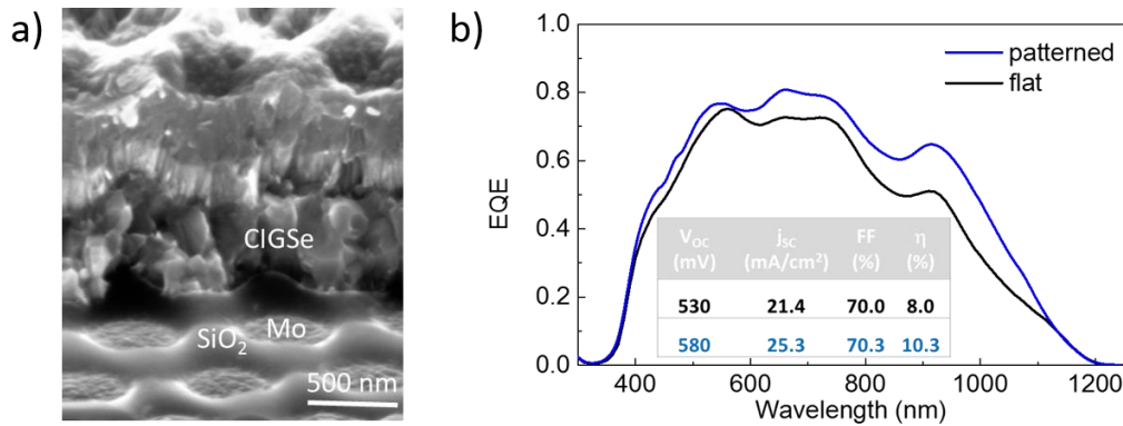
Figure 4. a) SEM cross-section of an ultra-thin Cu(In,Ga)Se 2 solar cell on top of a SiO 2 network, b) corresponding EQE as compared to planar reference.
