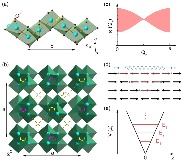
FIG. 1: (a) Screw chain consisting of \text{CoO}_6 octahedra running along the crystalline c axis in \text{SrCo}_2\text{V}_2\text{O}_8 . (b) Projection of left- and right-handed screw chains in the tetragonal ab plane. Interchain exchange interaction is dominated by the antiferromagnetic interaction J' between the nearest-neighbor Co ions in the ab plane, which are from the neighboring chains with the same chirality. (c) Shaded area indicates the excitation continuum of the spinon-pair quasiparticles corresponding to the Ising-like XXZ Hamiltonian in Eq. (1).[9] The spinon-pairs follow a quadratic dispersion relation along the chain direction close to the reciprocal \Gamma point ( Q_z = 0 ).[4, 9] (d) Magnetic excitations of spinon-pairs with total pseudospin \tilde{S} = 1 corresponding to an odd number of pseudospin-1/2 flips. The collinear antiferromagnetic order along the c axis is stabilized below 5 K.[5] (e) Quantized spinon-pair excitation levels due to linear confinement imposed by interchain exchange interaction.
