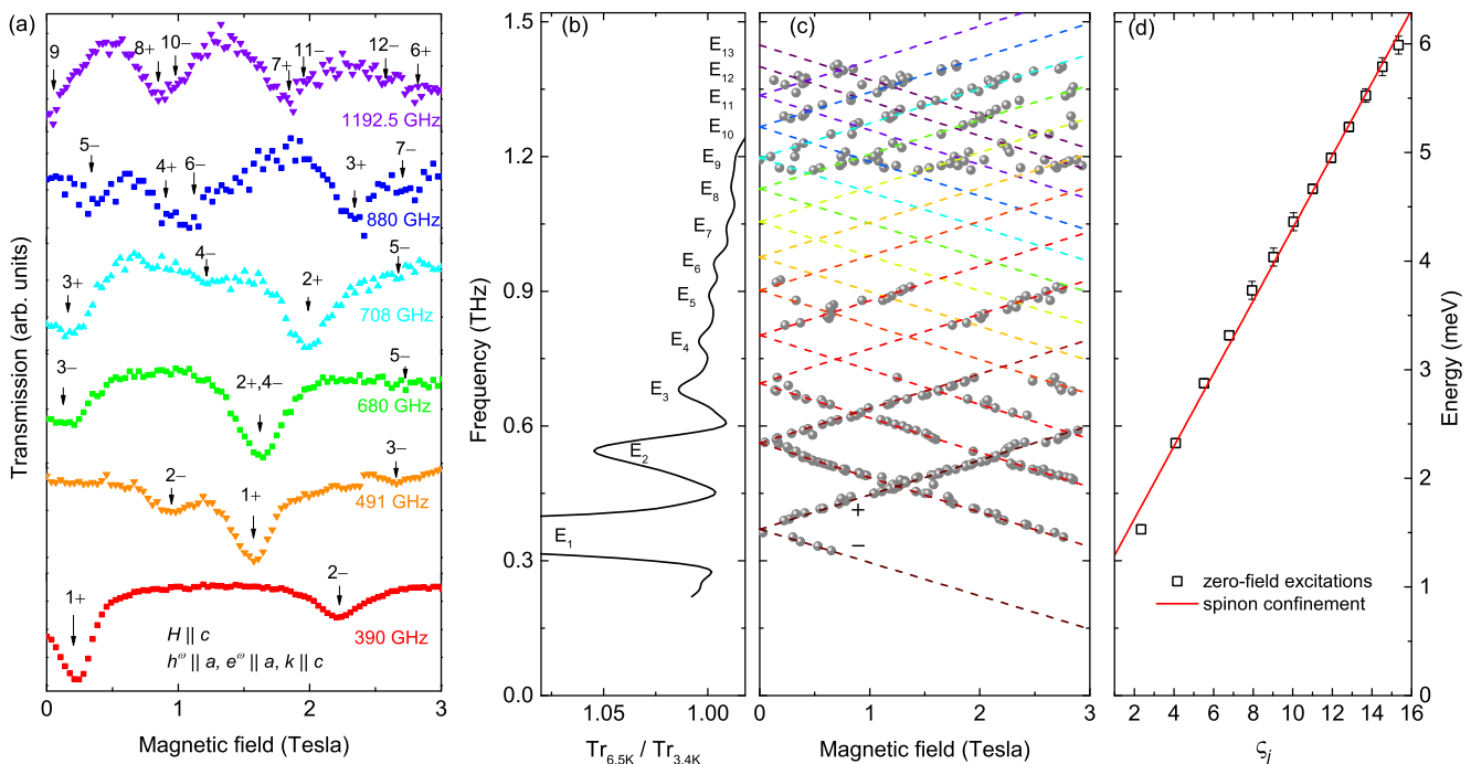
FIG. 3: (a) Transmission spectra of various frequencies as a function of a longitudinal magnetic field at 2 K. Absorption modes are marked by the corresponding number of energy level in Fig. 2(b). (b) Normalized transmission spectrum at zero field adapted from Fig. 2(c). (c) Energies of absorption modes as a function of applied longitudinal magnetic field. Their field dependence can be described by linear Zeeman term with a single g -factor g_{\parallel} = 5.5 (see text). (d) Hierarchy of the excitation energies at zero field can be modeled by the one dimensional Schrödinger equation with linear confinement Eq. (2). \zeta_j s are the negative zeros of the Airy function (see text).
