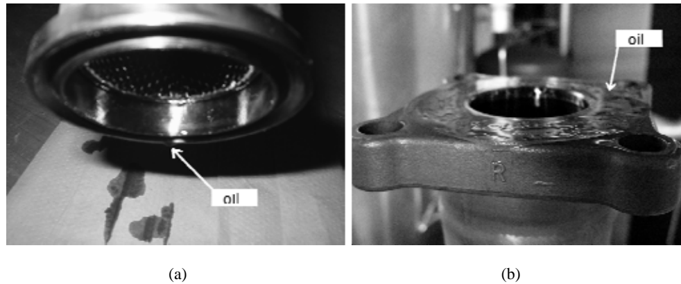
FIGURE 2. Oil residues inside the high pressure line of a LINDE TCF50 liquefier. (a) Coldbox inlet filter, (b) Flange of the ball valve downstream the charcoal adsorber.
