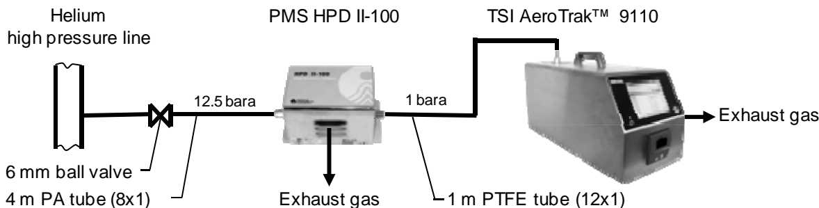
FIGURE 4. Particle measurement setup.
