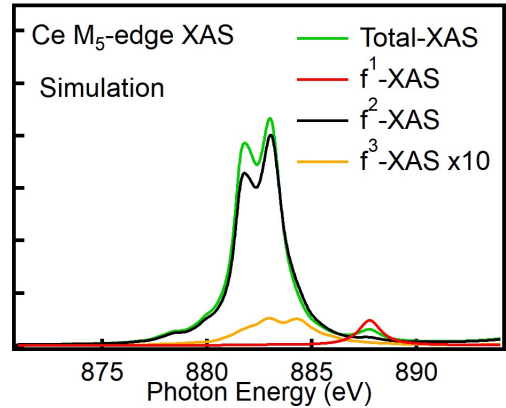
FIG. 7. Calculated XAS spectra at Ce-M5 edge and the contribution associated with the different configurations ( d^{10}f^0 \rightarrow d^9 f^1 , d^{10}f^1\bar{L} \rightarrow d^9 f^2\bar{L} and d^{10}f^2\bar{L}^2 \rightarrow d^9 f^3\bar{L}^2 ). It should be noted that the total XAS is not the sum of f^1 , f^2 , and f^3 contributions due to interference effects.
