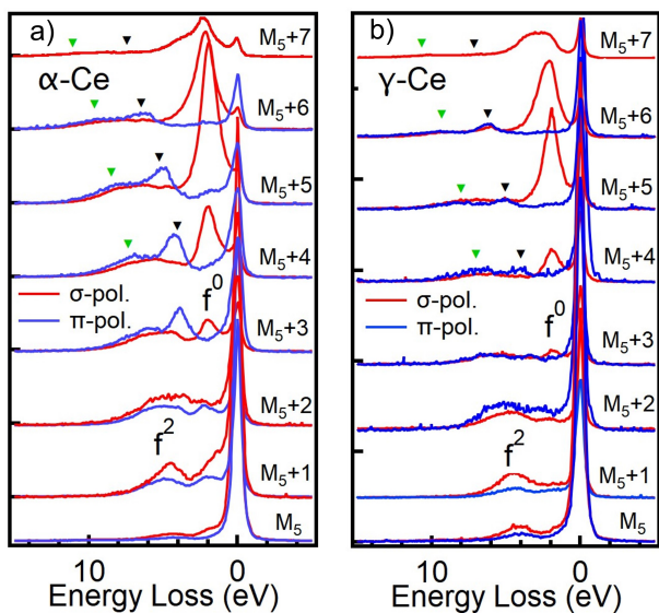
FIG. 2. Ce 3d \rightarrow 4f \rightarrow 3d RIXS spectra of \text{Ce}_{0.93}\text{Sc}_{0.07} as a function of the energy loss. The measurements were performed at (a) T = 20 K ( \alpha -phase) and (b) T = 300 K ( \gamma -phase) in \sigma and \pi polarizations. The incident photon energy is tuned in steps of 1 eV of the XAS spectrum, starting with M_5 up to M_5 + 7 (2 eV above the f^1 XAS satellite). (see figure 1). M_5 denotes the excitation energy, which coincides with the maximum of the XAS spectrum ( h\nu = 883 eV). The green and black triangles indicate two different fluorescence-like features.
