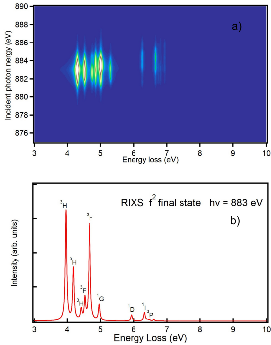
FIG. 8. (a) RIXS map in the energy loss range of the f^2 final state. (b) RIXS spectra at h\nu = 883 eV.
