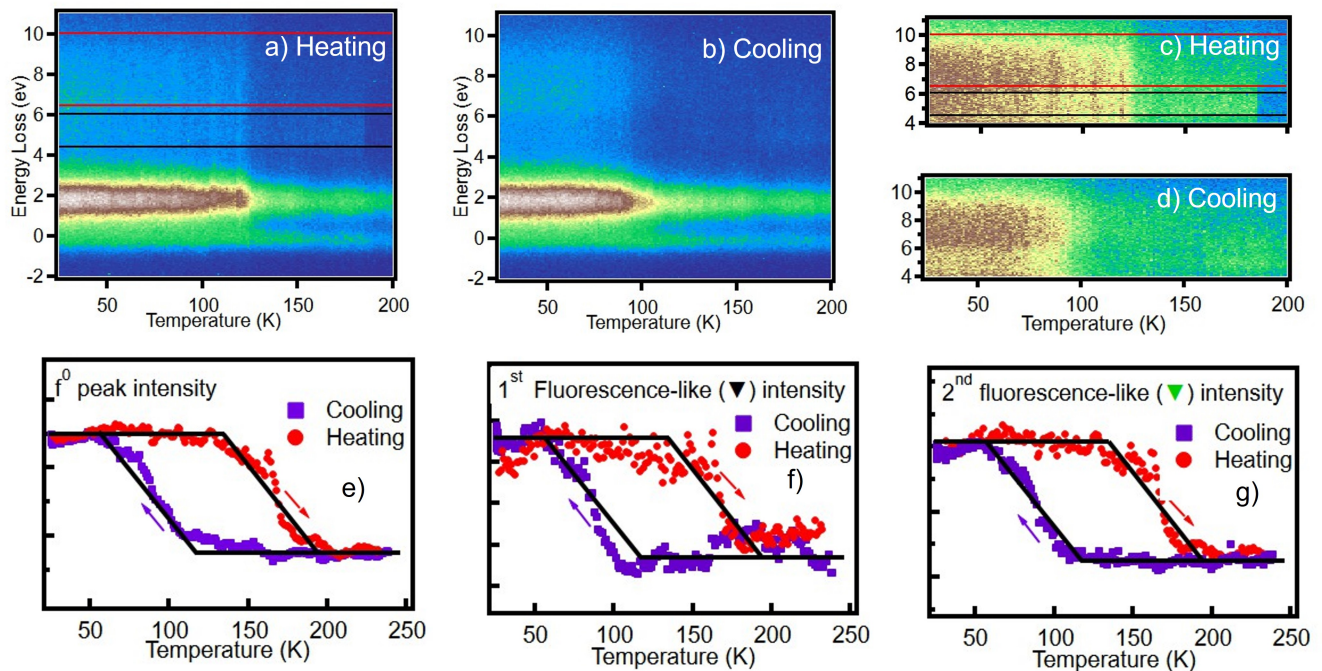
FIG. 4. (a-d) Highlighting of the \gamma - \alpha transition with the T -dependent RIXS map measured in \sigma polarization with the incident photon energy h\nu = M_5 + 5 ((c) and (d) are the RIXS map expanded in the region of the fluorescence feature). Hysteresis loops derived from the integrated intensity of the (e) f^0 , (f) first and (g) second fluorescence-like structure (indicated by the black and green triangles in Figure 2) in the RIXS map of \text{Ce}_{0.97}\text{Sc}_{0.07} (see figures 4a and 4b). The arrows indicate the circulation inside the loop.
