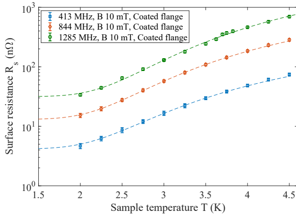
Figure 6: R_S vs. T for the coated flange at three quadrupole modes. R_{\text{res}} is extrapolated from fits using Eq. (1).
