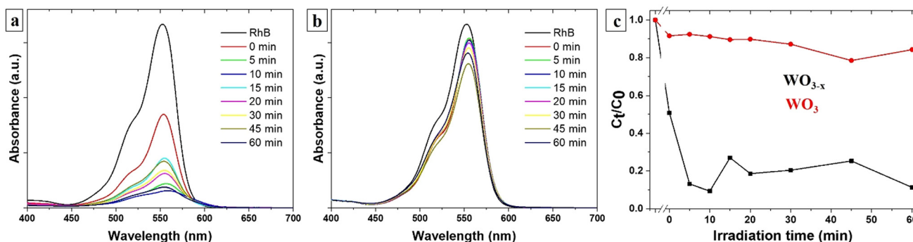
Fig. 7 (a) UV-Vis absorption spectra of RhB solutions at a pH of 2.5, containing the \text{WO}_{3-x} nanowires as photocatalysts after different solar irradiation times. (b) UV-Vis absorption spectra of RhB solutions at a pH of 2.5, containing the \text{WO}_3 nanowires as photocatalysts after different solar irradiation times. (c) Photodegradation ratio vs. irradiation times for both samples.
