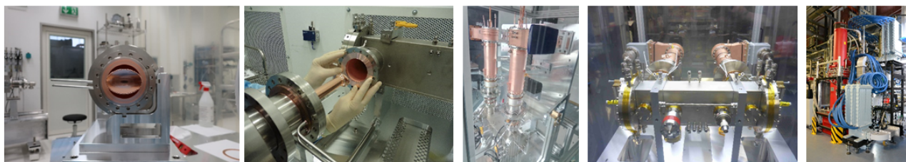
Figure 2: Overview of the steps taken from cleanroom assembly to final setup at test location of the conditioning set up.
