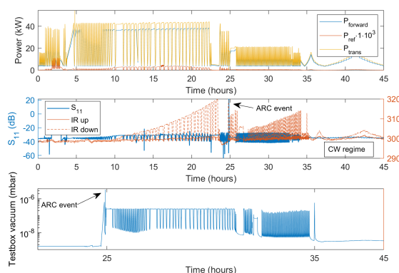
Figure 7: Part of the conditioning series of the 2 nd coupler pair displaying peak power, S_{11} parameter, ceramic window temperatur and testbox vacuum with time.
