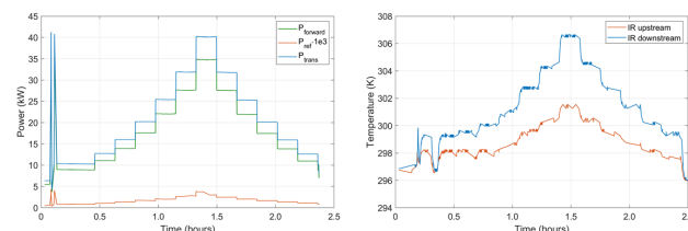
Figure 5: CW power ramps in traveling wave mode with corresponding heating at the ceramic windows measured by infrared sensors.
