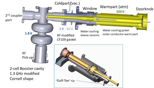
Figure 1: Schematic overview of the bERLinPro Booster injector coupler. The insert gives an better view on the Golf-Tee shaped antenna tip and the doorknob transition.
