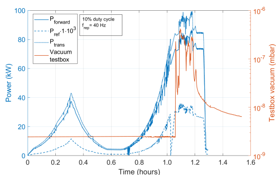
Figure 4: Intermediate result of first condition series with 1 st pair reaching about 90 kW forward power at 10 % duty cycle with 40 Hz repetition rate displaying the three power signals and testbox vacuum with time.
