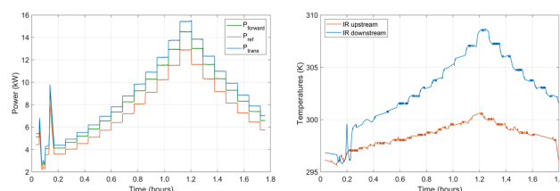
Figure 6: CW power ramps in standing wave mode with corresponding heating at the ceramic windows measured by infrared sensors.
