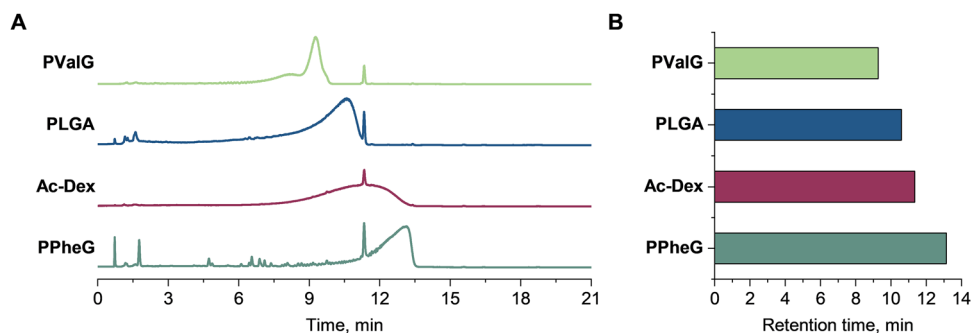
Fig. 2 (A) Overlay of normalized elution traces of polymers recorded by a charged aerosol detector (CAD). (B) Polymer elution times determined as a first moment of the distribution (peak). Conditions: Chromolith ® High Resolution RP-18 endcapped column (100 × 4.6 mm), gradient elution programming: the mobile phase composition was kept constant at 50/50 (% v/v) CH 3 CN/H 2 O for 1 min, followed by an increase of CH 3 CN content to 100% within 10 min and an isocratic hold at 100% CH 3 CN for 8 min. Flow rate: 1.0 mL min -1 . Column temperature: 30 °C. Injection volume: 5 μL. The polymers were dissolved in 50/50 DMSO/CH 3 CN (% v/v) at a concentration of 1 mg mL -1 .
