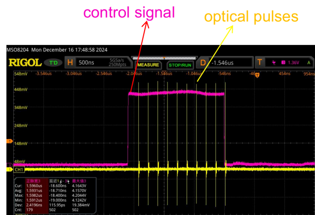
Figure 1: Output of the PoP II laser: Macropulses emitted at a repetition rate on the order of 1 Hz consist of a variable number of micropulses emitted at 6.25 MHz (yellow). The laser supplies a control signal outlining the macropulse to trigger the detection setup (pink).
