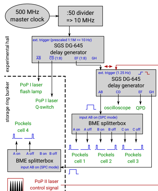
Figure 6: Sketch of the triggering scheme enabling both PoP I and PoP II laser operation. To switch between the laser systems, the input trigger of the second delay generator has to be exchanged (red arrow).
