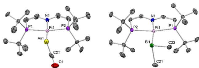
Figure 2. Molecular structure of 1^{\text{Pt,As}} (left) and 1^{\text{Pt,Bi}} (right) with thermal ellipsoids at the 50% probability level. H atoms are omitted for clarity. Selected bond lengths [Å] and angles [°]: 1^{\text{Pt,As}} Pt1–As1:2.455(1); Pt1–As1–C21:99.0(3); 1^{\text{Pt,Bi}} : Pt1–Bi1:2.7323(3); Pt1–Bi1–C21:99.69(15), Pt1–Bi1–C22:117.53(14), C21–Bi1–C22:91.7(2).
