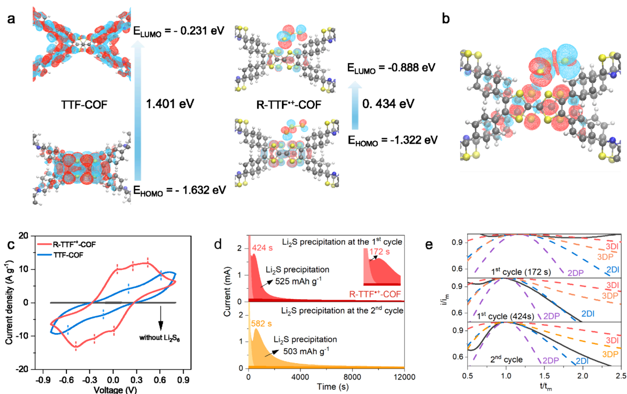
Figure 3. Electronic structures and catalytic properties of R-TTF + -COF. (a) HOMO/LUMO distributions of the adjacent bilayer molecular units in TTF-COF and R-TTF + -COF and their corresponding energy levels. (b) The spin density plots of R-TTF + -COF calculated via DFT by consideration of the interaction between neighboring [TTF] 2 •+ and S 3 •- , where the red region designates \alpha -spin, and the blue region designates \beta -spin. (c) CV curves of symmetric cells in the voltage window of -0.8 – 0.8 V at a scan rate of 5.0 mV s -1 in Li 2 S 6 electrolyte. (d) The potentiostatic Li 2 S precipitation process at 2.05 V on an R-TTF + -COF electrode at the first and second cycles. (e) The corresponding dimensionless transient of R-TTF + -COF electrode at the first and second cycles fitted with theoretical 2D/3D models, respectively ( t_m denotes the time needed to reach the peak current, i_m denotes the peak current).
