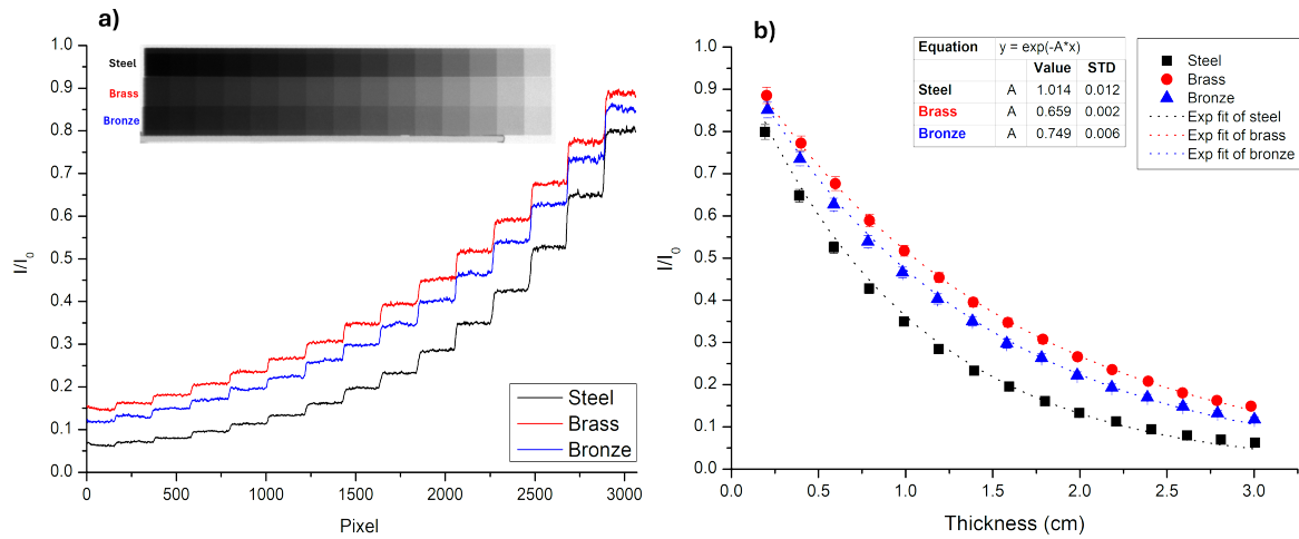
Figure 2. a) Radiography and transmission profile of the three step wedges; b) neutron attenuation curves for the three wedges as a function of the step thickness.
