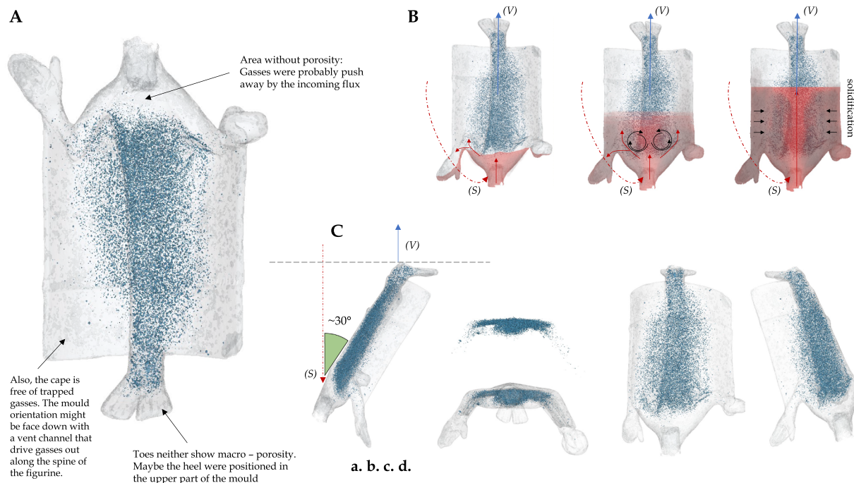
Fig. 10. Casting hypothesis of the statuette. (A) In the main body of the statuette, the accumulation of porosity is shown in turquoise: the black arrows point to the areas of the object that appear without pores. Based on the confinement of the pores, it is possible to hypothesize that direct lost wax casting was used exploiting a duct that allowed the mould to be filled from bottom upwards (B). Consequently, the figure may have been cast upside down with a main sprue (S) at shoulder height and a ventilation channel (V) positioned above the feet (C). If we then consider the abrupt vertical interruption of the pores at the height of the shoulder blades (C, a.), and the fact that the farthest point reached by the porosity is in the heels, we can assume that the mould may have been positioned tilted ( \sim 30^\circ ).
