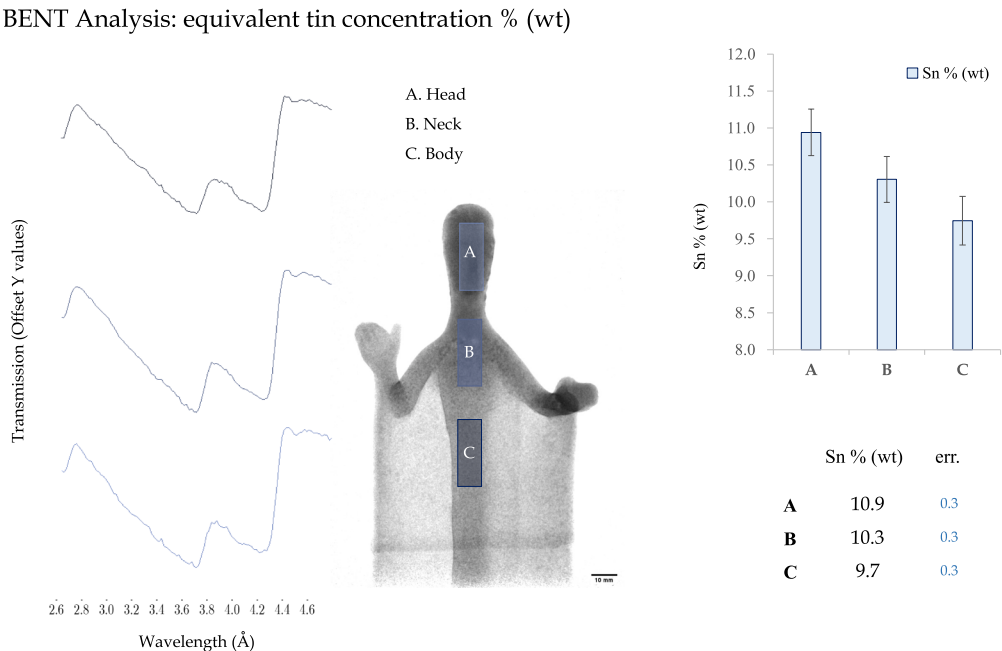
Fig. 9. Results of the BENT analysis conducted on the statuette, showing the equivalent tin content (% wt) of three sample volume A, B and C (10 mm x 10 mm x 20 mm) of the statuette, obtained from the corresponding transmission plots.
