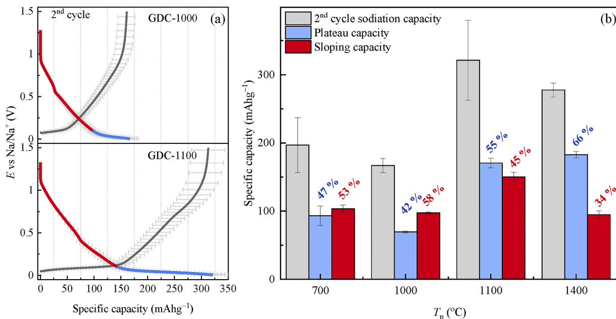
Fig. 1. (a) Sodiation-desodiation of electrochemical half-cells during the second cycle, featuring GDC-1000 (above) and GDC-1100 (below) HC anodes (Data normalisation is given in Table S2 in SI). The sodiation curves are divided into two regions: the sloping region (red line, E > 0.1 V) and the plateau region (blue line, E < 0.1 V). (b) The ratio of second-cycle sloping and plateau capacities in electrochemical half-cells constructed with hard carbon anodes synthesised at various pyrolysis temperatures.
