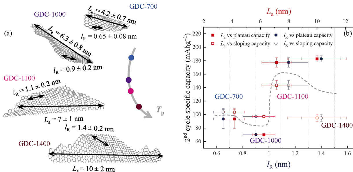
Fig. 5. (a) The diagram illustrating the alterations in the graphene layer in the studied HCs as a function of the T_p according to the obtained L_a and l_R parameters. (b) Empirical correlations between the L_a and l_R parameters and the second cycle sodiation plateau- and sloping specific capacities.
