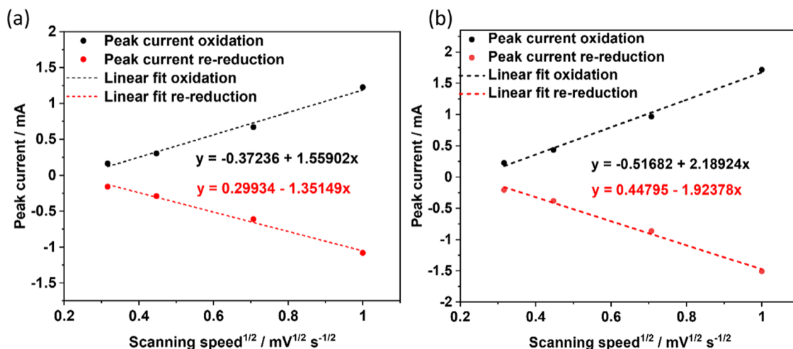
Figure 5. Plot of the peak currents vs the square root of the scanning speeds from the cyclic voltammetry analysis of the batteries during the CV testing. (a) Hydrogel electrolyte and (b) liquid electrolyte containing \text{Zn}(\text{ClO}_4)_2 with a glass fiber separator. Linear fit.
