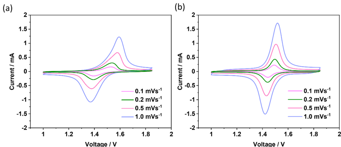
Figure 4. Cyclic voltammetry measurements of PTMAM/Zn coin cells at 0.1, 0.2, 0.5, and 1.0 \text{mVs}^{-1} scanning rates and different electrolytes. (a) Hydrogel electrolyte and (b) liquid electrolyte containing \text{Zn}(\text{ClO}_4)_2 with a glass fiber separator.
