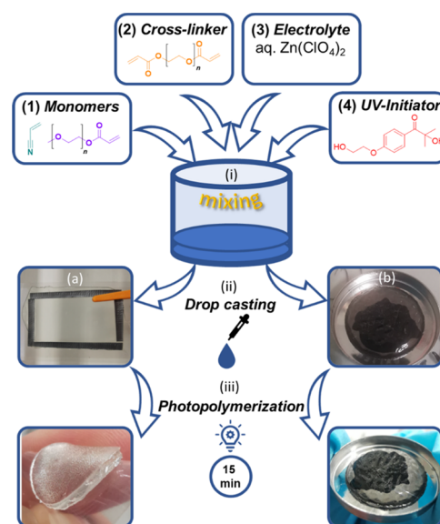
Figure 1. Preparation of the hydrogel electrolyte. (i) Mixing of monomers, UV initiator, and aqueous electrolyte solution, (ii) (a) drop-casting onto the Mylar film in a frame to produce a free-standing hydrogel, (b) drop-casting directly onto the cathode surface, and (iii) UV polymerization in a UV cube during 15 min.
