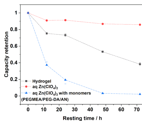
Figure 7. Percentage of retained capacity after self-discharge for the PTMAM/Zn batteries with (black) hydrogel electrolyte and (red) aq. Zn(ClO 4 ) 2 and (blue) aq. Zn(ClO 4 ) 2 with monomers (PERMEA/AN/PEG-DA) at different resting times.
