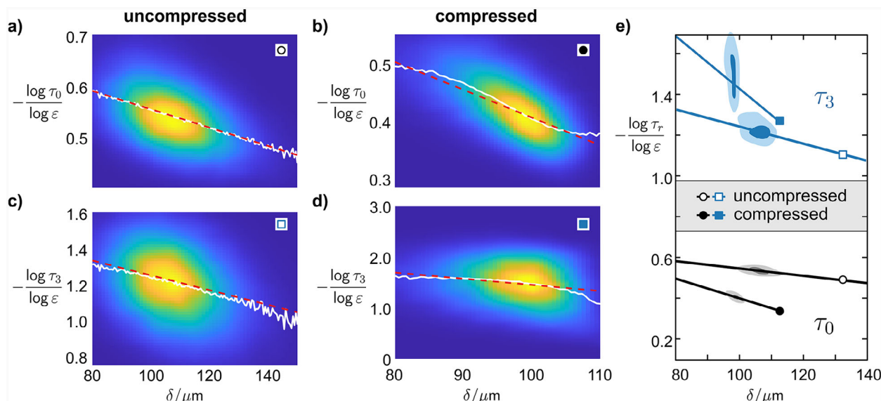
Figure 8. Dependency of the exponent a = -\log \tau_r / \log \varepsilon on the local thickness \delta , shown for a,c) uncompressed and b,d) compressed paper sheets by the bivariate probability density of (a, \delta) (heatmap), together with the conditional mean values of a for given values of \delta (white curves) and its linear fit (dashed lines). Left panels (a,c) concern the tortuosity \tau_0 (i.e., r = 0 ) with respect to all paths, while the middle panels (b,d) refer to tortuosity \tau_3 with respect to high volume paths ( r = 3 ). e) The right panel shows a comparison of the linear relation between a and \delta for all four cases on equal length scales. As a guide to the eye, the regions with high probability in (a–d) are indicated.
