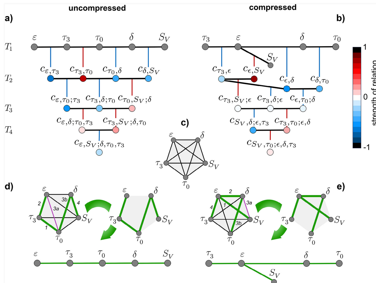
Figure 5. a,b) Tree representation of pair copula decomposition obtained by fitting R-vine copulas to the multivariate distribution of the local descriptors porosity \epsilon , sheet thickness \delta , surface area per unit volume S_V and path-length related descriptors \tau_0 and \tau_3 . Tree representations are shown for uncompressed (a) and compressed (b) paper sheets. Colored vertices of trees T_2 , T_3 and T_4 indicate the size and sign of Kendall's tau \tau_K . c–e) Determination of the material-specific order of descriptors in tree T_1 using maximum spanning trees for the d) uncompressed and e) compressed paper sample. c) Graph in which descriptors are vertices arranged as in the random vector W = (\epsilon, \delta, S_V, \tau_0, \tau_3) and all pair-wise connections represented as edges. (d,e) Shows how the maximum spanning tree for the graph (c) is determined by connecting descriptors with strongest pair-relations in descending order.
