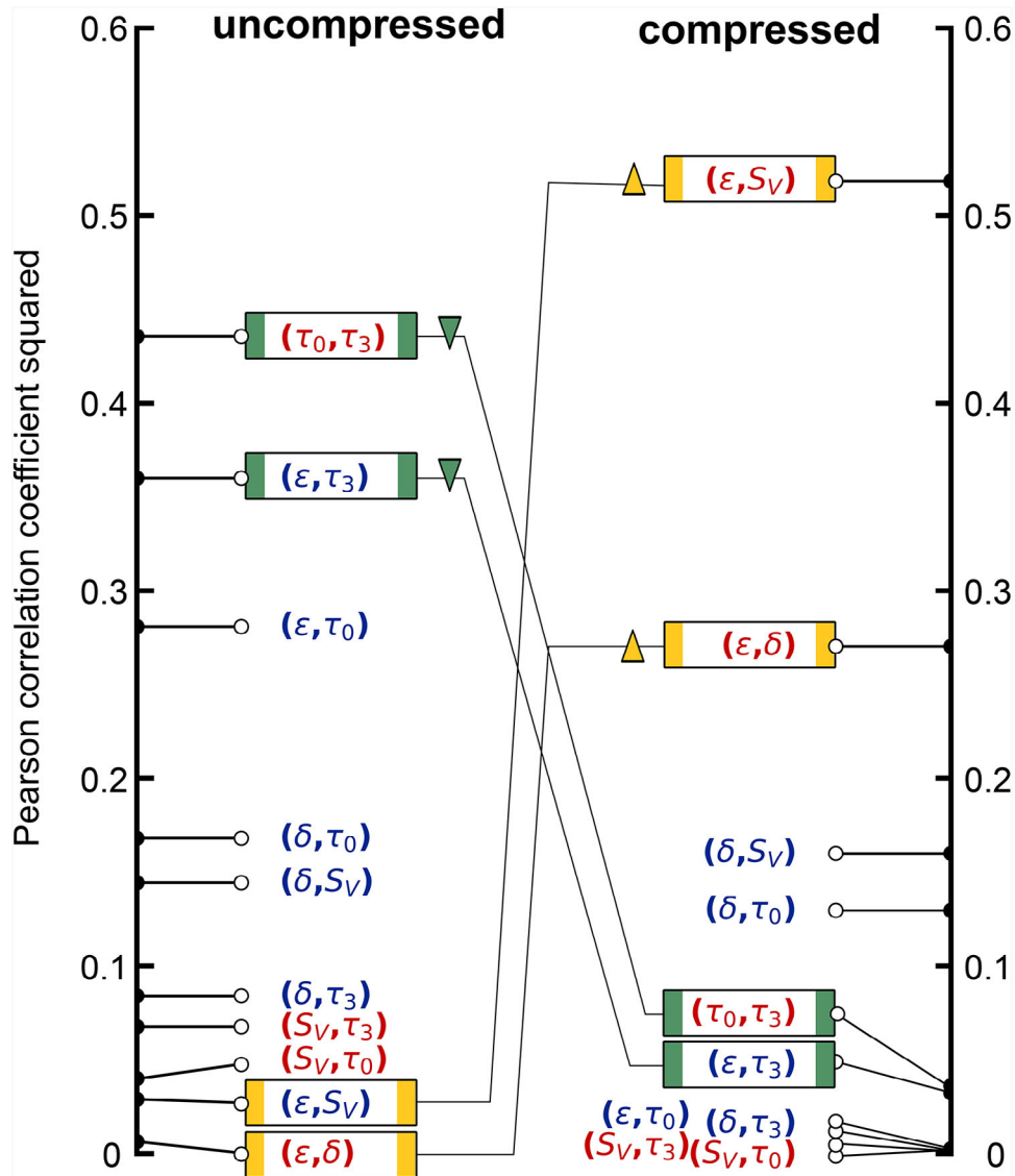
Figure 3. Pairwise Pearson correlation coefficients squared for porosity ( \epsilon ), sheet thickness ( \delta ), specific surface area ( S_V ), and the two path-length related descriptors \tau_0 and \tau_3 for the uncompressed (left) and compressed (right) paper sheets. Labels in red indicate positive correlations, labels in blue negative correlations. To guide the eye through changes in correlations upon compression, some property pairs are highlighted with a box. Green bars (down triangles) indicate pairs, whose relations weaken after compression; yellow bars (up triangles) indicate pairs with increased dependence after compression.
