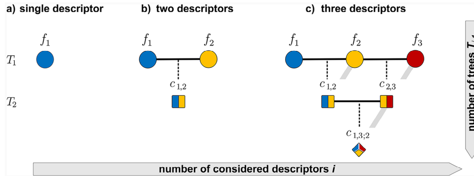
Figure 4. Pair copula decomposition of f represented by graphs for the example of a) one, b) two and c) three correlated descriptors. Each vertex in a graph corresponds to a density function that enters the vine copula of f as a factor. Edges indicate a dependence between two descriptors. As a guide for the eye, all factors associated to a new descriptor added are connected with a diagonal, grey bar. Each new descriptor extends the scheme to the right via factors (vertices) aligned along such a diagonal and adds a new tree T_{i-1} if i \geq 2 .
