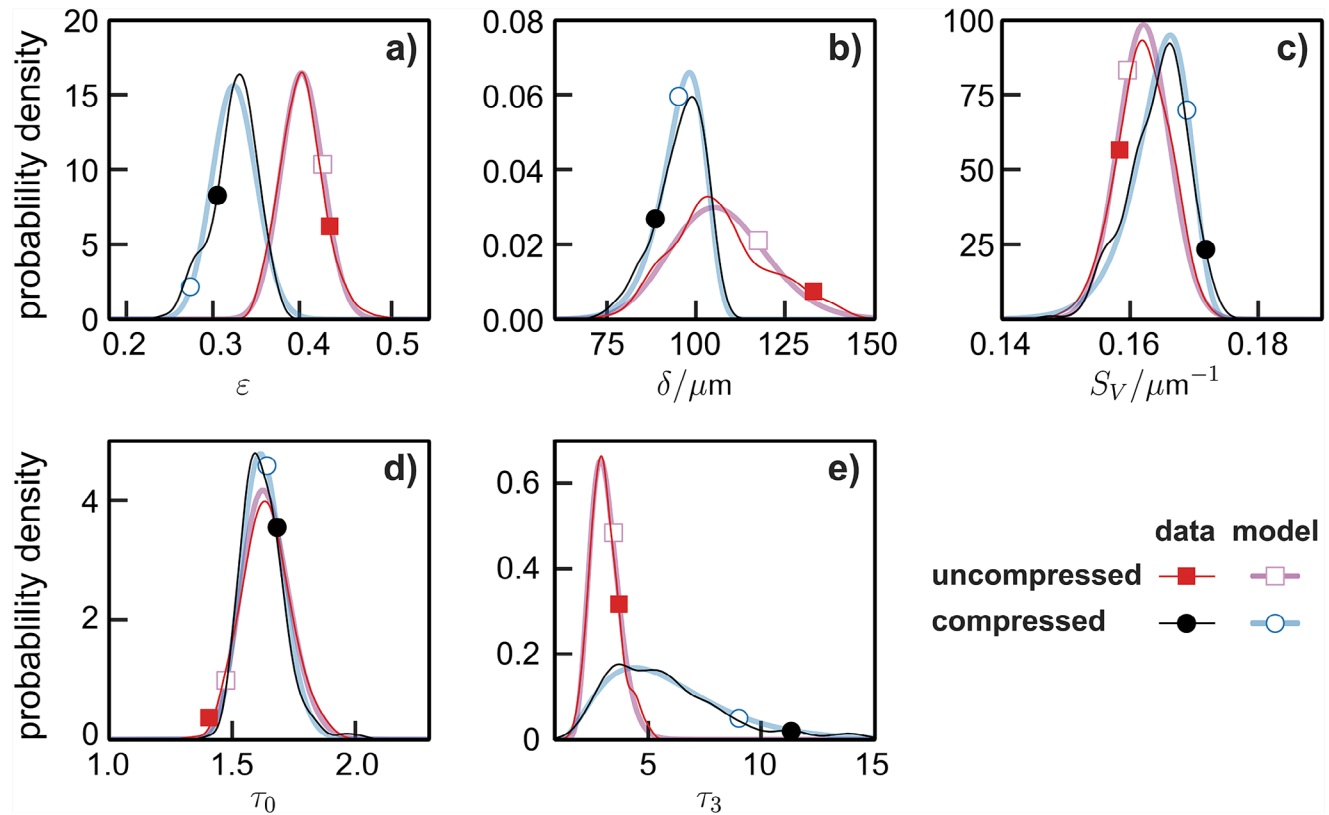
Figure 2. Univariate density functions of microstructure a) descriptors porosity \varepsilon , b) sheet thickness \delta , c) specific surface area S_V , as well as d) the means geodesic tortuosities \tau_0 , and e) \tau_3 for the uncompressed and the compressed paper sample. The densities of microstructure descriptors computed from 3D image data via kernel density estimation (filled symbols) are compared with the corresponding parametric model densities (open symbols).
