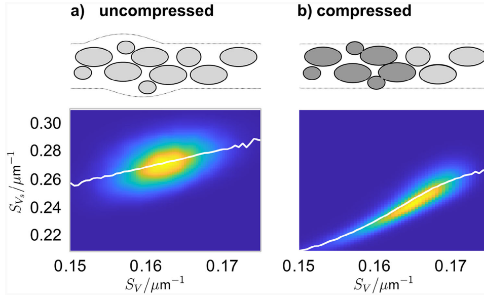
Figure 7. Comparison of a) uncompressed and b) compressed paper sheets to reveal the impact of compression on the relation between local surface area per unit volume, S_V , and local surface area per solid volume, S_{V_s} . For both paper sheets, the arrangement of fibers (gray) in a cross-section of a sheet is schematically visualized. The bold contour of the cross-sections of fibers indicate their contributions to the local surface area. In the compressed paper (b), compacted regions are indicated with fiber cross-sections shaded in dark-gray. The joint probability density of S_{V_s} and S_V is shown as heatmap. The white curves indicate how the (conditional) mean value of S_{V_s} changes with the value of S_V .
