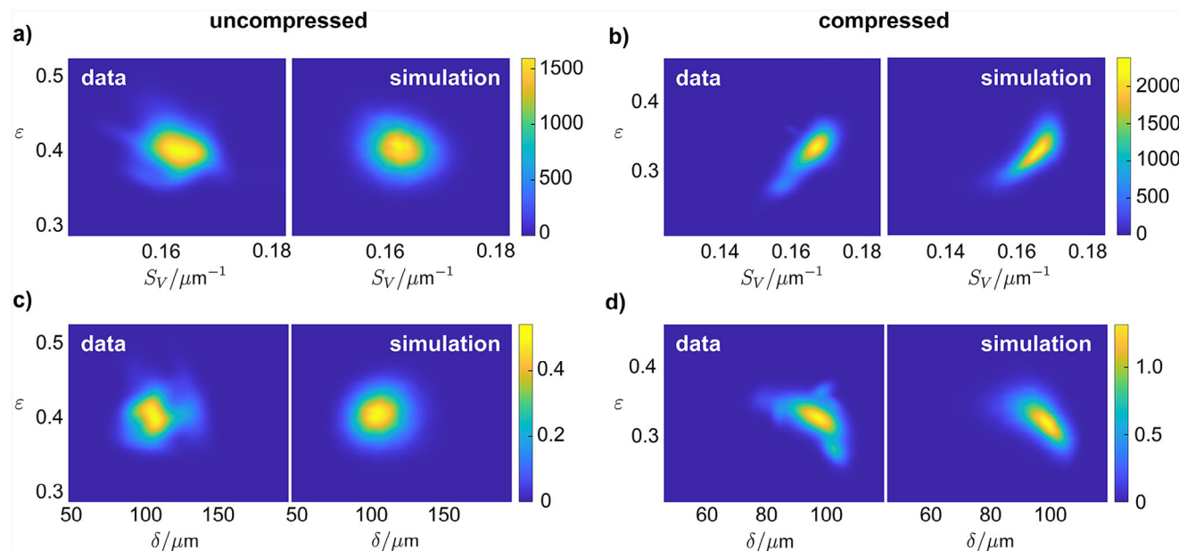
Figure 6. Bivariate probability densities of a,b) porosity \epsilon and specific surface area S_V , and of c,d) porosity \epsilon and sheet thickness \delta (c,d), each shown for the a,c) uncompressed and b,d) compressed paper sheets. For each case, the bivariate density obtained via kernel density estimation is shown for measured image data (left) and simulated data drawn from the copula-based model (right).
