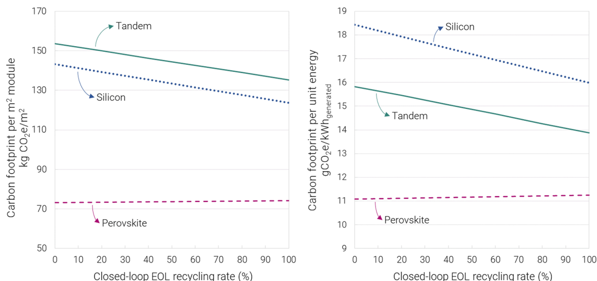
FIGURE 4 Carbon footprints (a) per \text{m}^2 module produced, and (b) per lifetime energy generated, normalized to an average irradiation of 1700 \text{ kWh}/(\text{m}^2 \text{ year}) , PR of 0.75, and a lifetime of 30 years. Breakdowns of Scope 1, 2, and 3 emissions can be found in Supporting Information S1 (Section S3, Figure S2) and all underlying data in Supporting Information S2.
