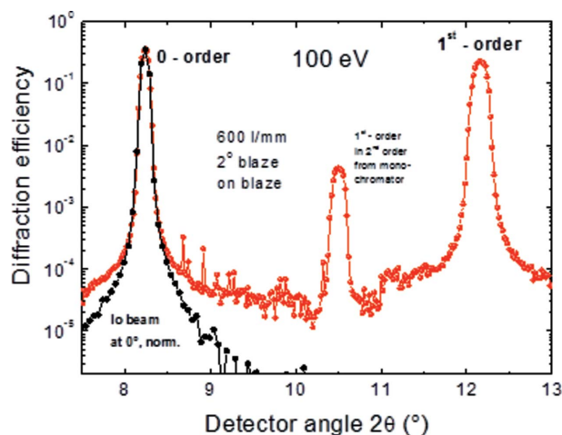
Figure 14 Diffraction efficiency of a blazed diffraction grating of 600 lines \text{mm}^{-1} in zero and first order at 100 eV, operated on-blaze. The Io-beam profile (shifted and normalized to the zero-order peak) is also shown for comparison (black points). Second-order radiation in the incident beam (photon energy 200 eV) which is not suppressed creates a first-order diffraction peak at 2\theta = 10.5^\circ .
