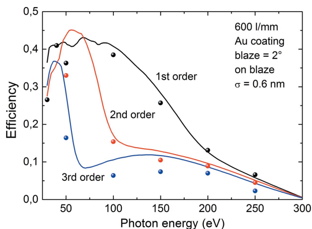
Figure 15 Integrated efficiencies of the 600 lines \text{mm}^{-1} blazed grating for the first, second and third order in comparison with calculation using REFLEC (Schäfers & Krumrey, 1996).
