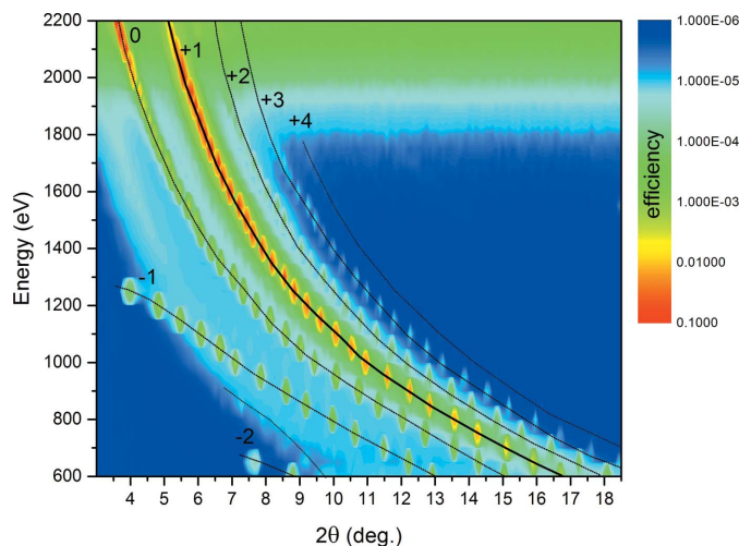
Figure 16 Two-dimensional map of the diffracted intensity (energy versus detector angle 2\theta ) of a Cr/C multilayer-coated blazed grating (2000 lines \text{mm}^{-1} ) recently produced at HZB for the soft X-ray range. All diffraction orders from -1 to 4 are visible (Senf et al. , 2016).
