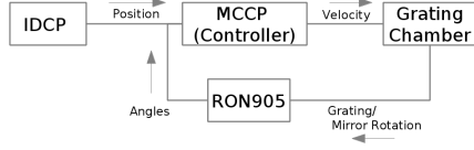
Figure 2: Feedback loop. Desired velocity profiles derived from the readback received from the undulator control program (IDCP). Monochromator position feedback from Heidenhain system (RON905).
